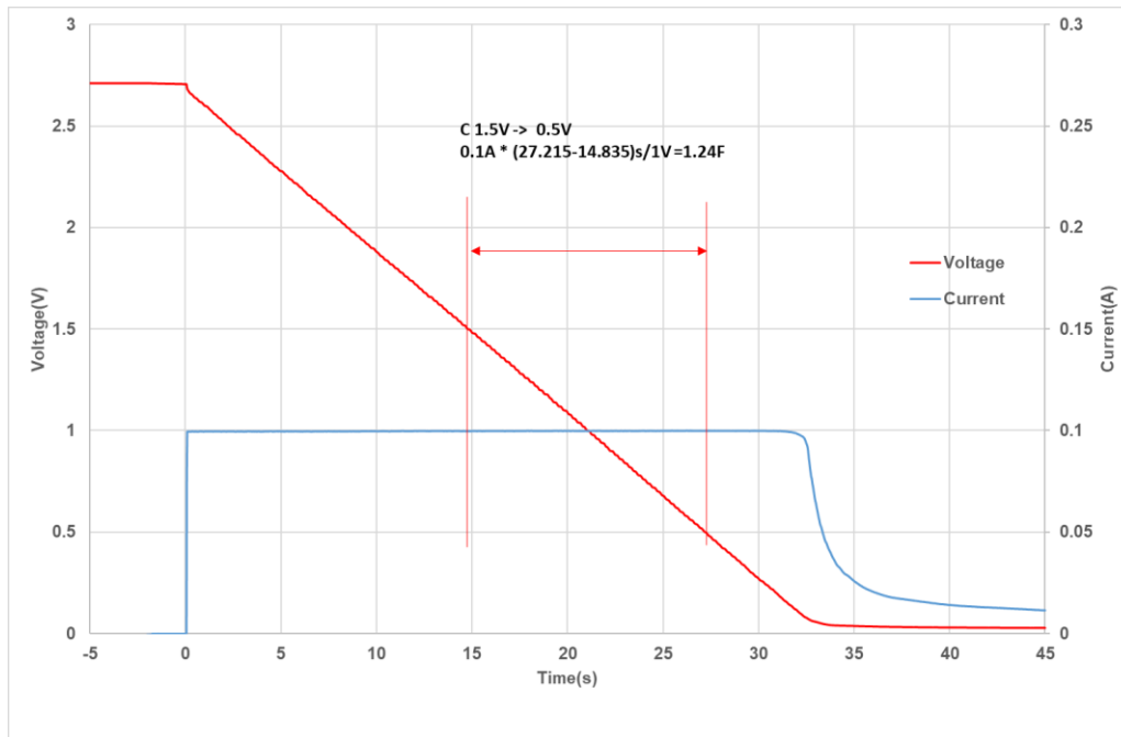
Fig 1: HY12R708012S105R Capacitance measurement
