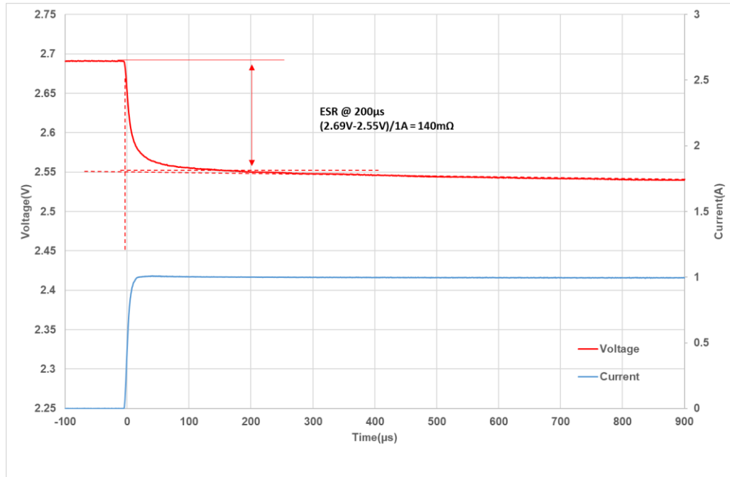
Fig 2: HY12R708012S105R ESR Measurement
