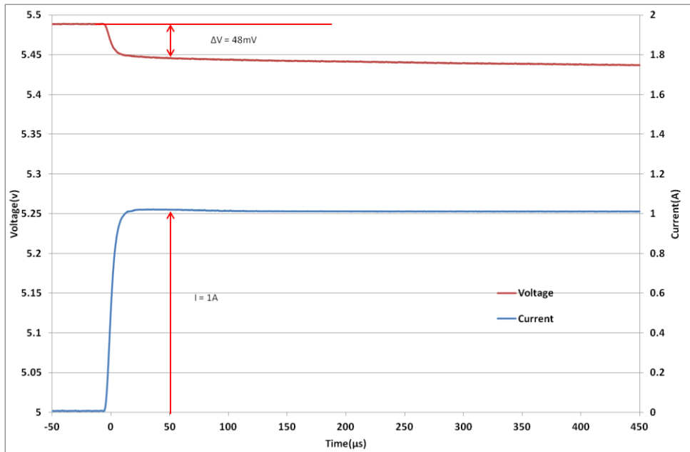
Fig 3: Measurement of ESR for an HS208
