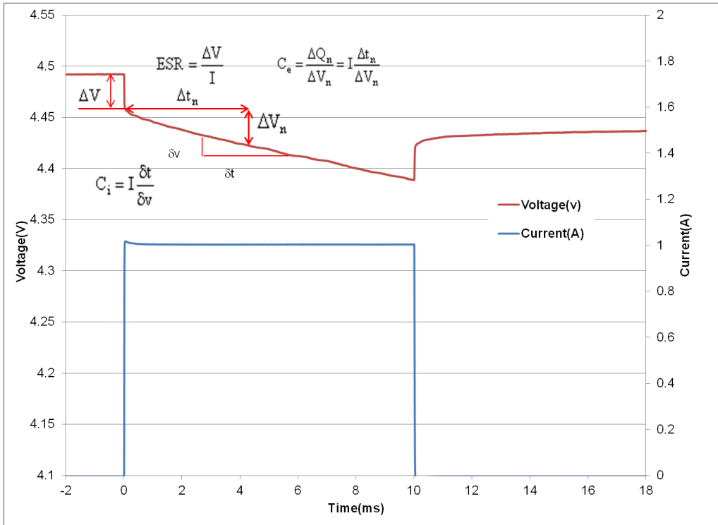
Fig 1: Effective capacitance, instantaneous capacitance and ESR for a GW202
