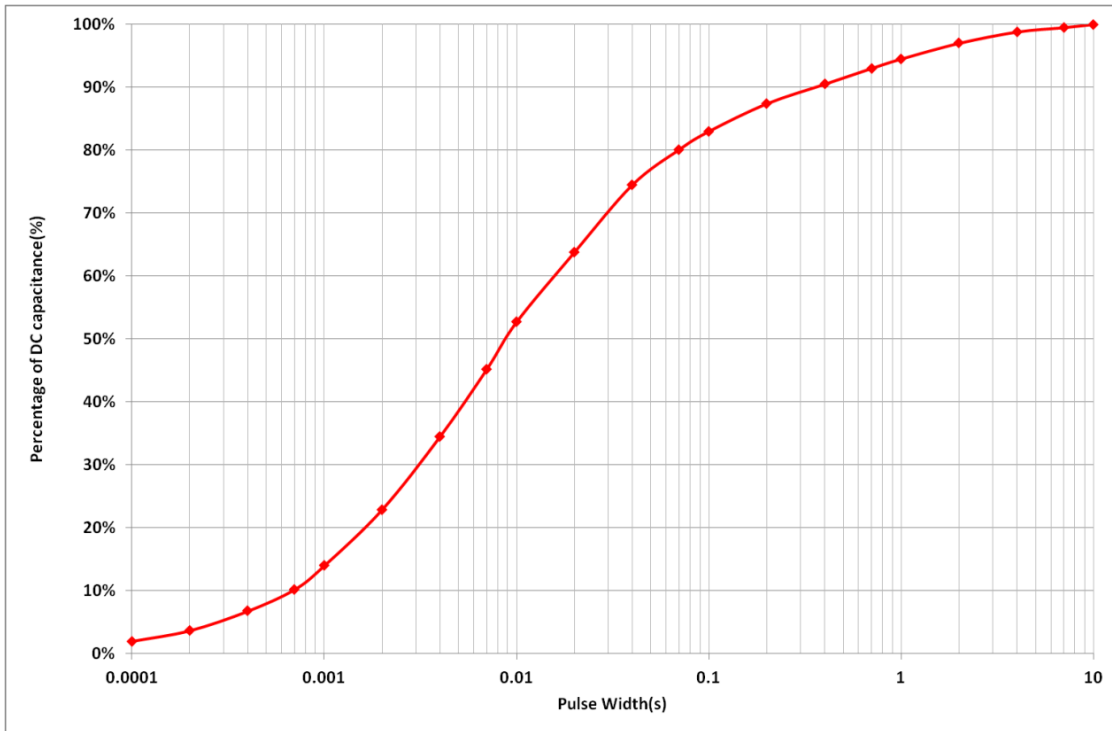
Figure 4: Effective Capacitance
