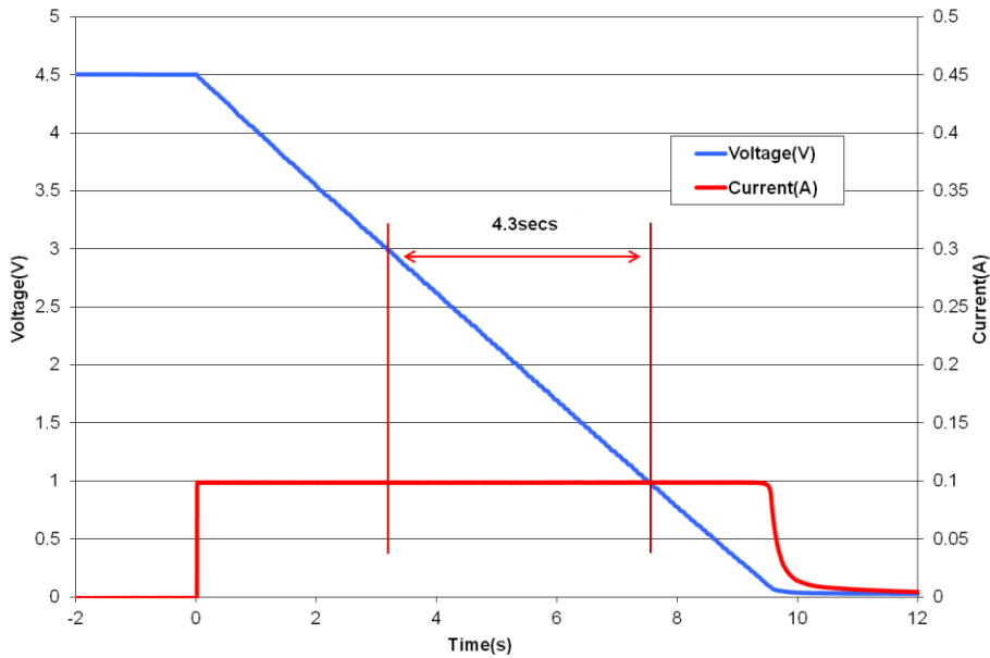
Fig 2: Measurement of DC Capacitance for a GW202
