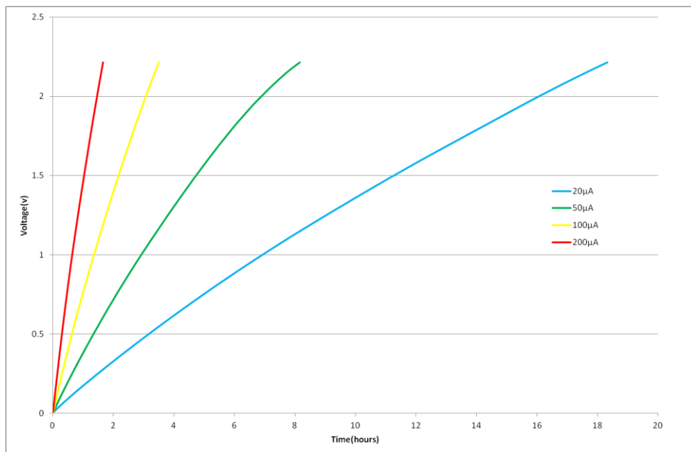
Fig 11: Charging a GW102 with low current
