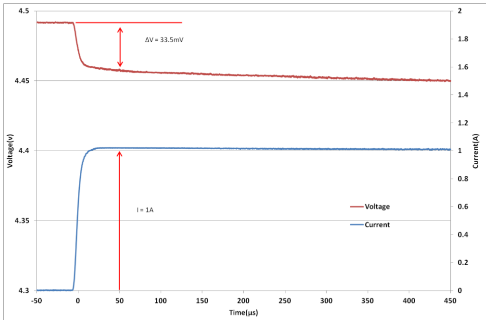
Fig 3: Measurement of ESR for a GW202
