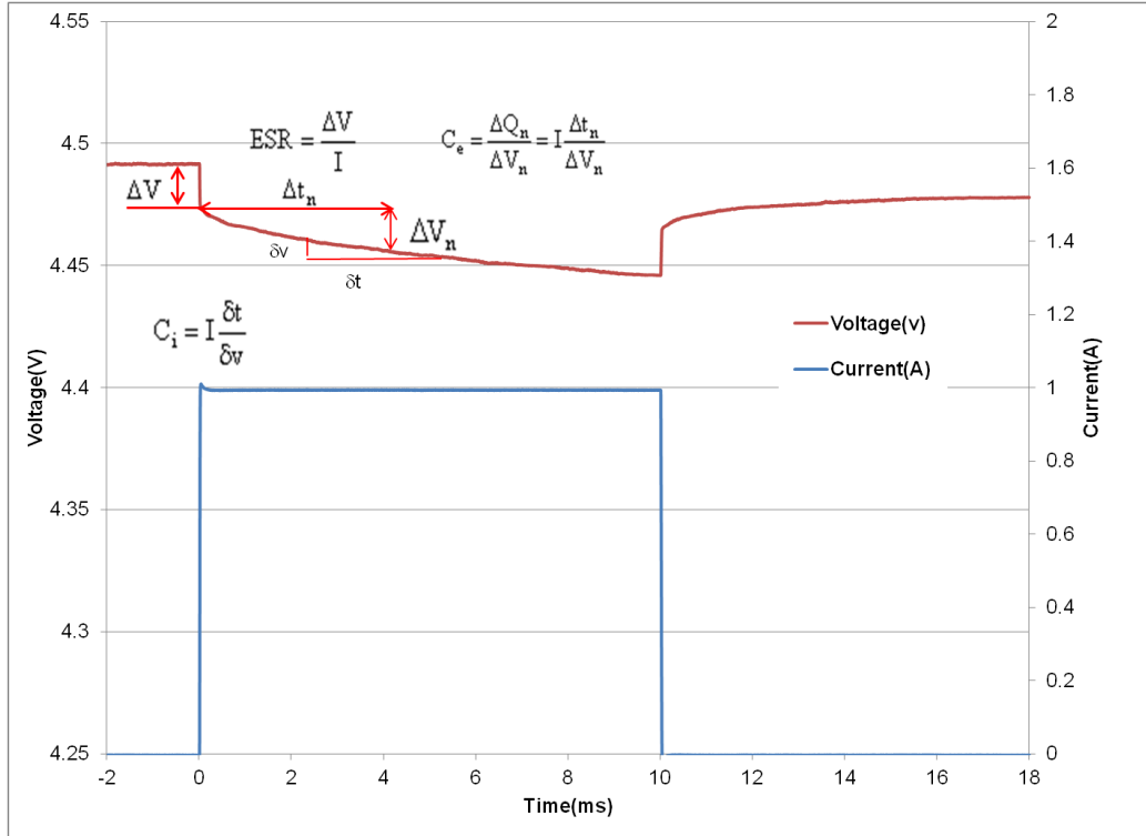
Fig 1: Effective capacitance, instantaneous capacitance and ESR for a GS208
