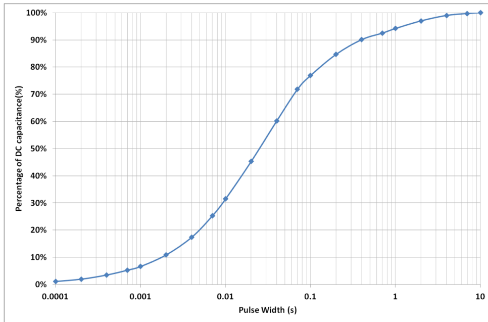
Figure 4: Effective Capacitance
