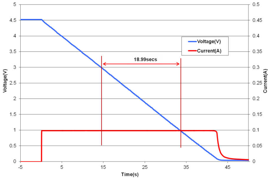
Fig 2: Measurement of DC Capacitance for a GS208
