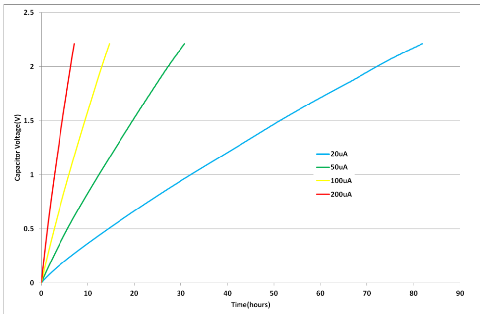
Fig 11: Charging an GS108 with low current
