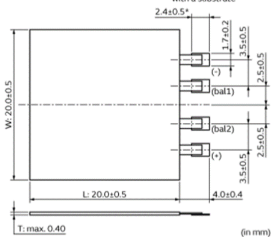
Mechanical drawing and recommended landing pad for DMHA14R5V353M4ATA0
