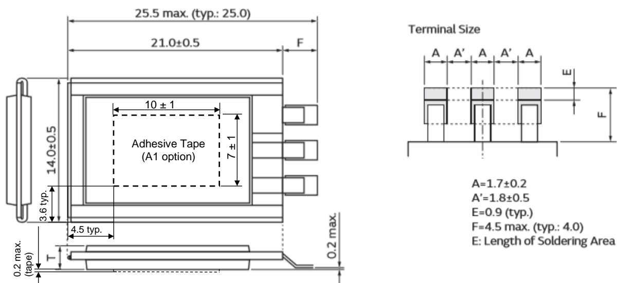
Mechanical drawing for DMT3N4R2U224M3DTA0
