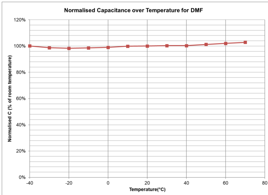
Fig 5: Capacitance change with temperature
