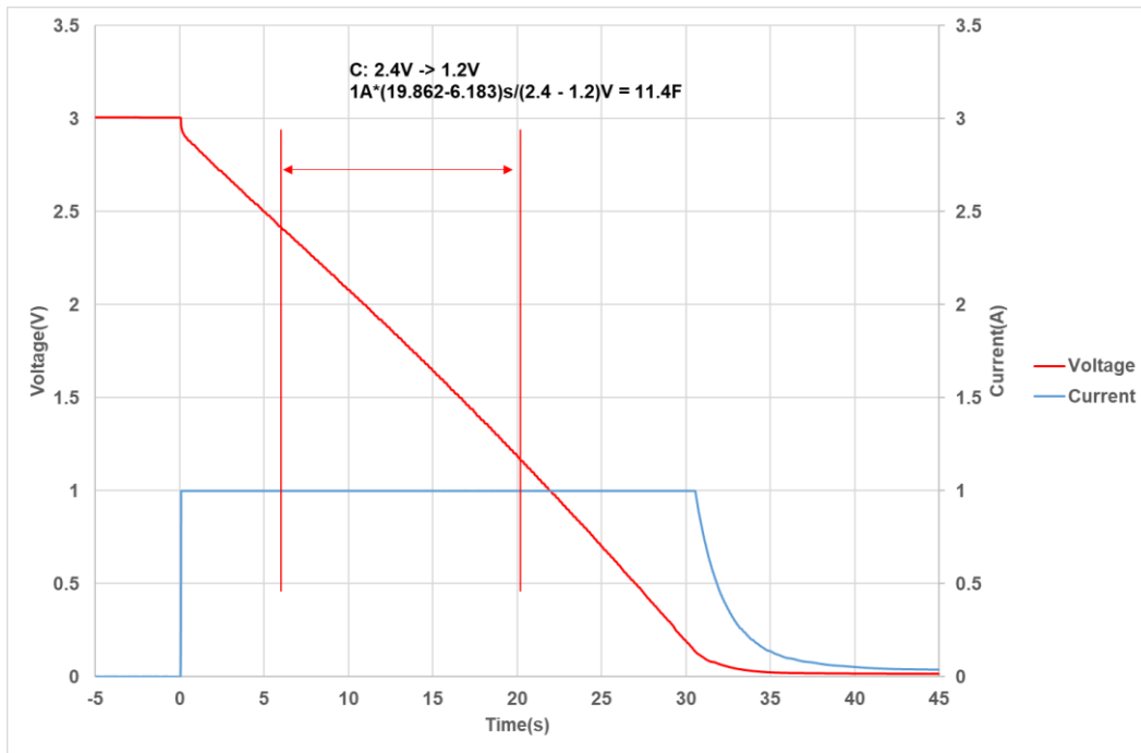
Fig 1: Capacitance measurement
