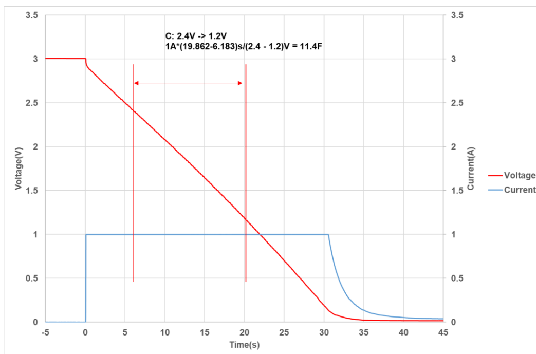
Fig 1: Capacitance measurement
