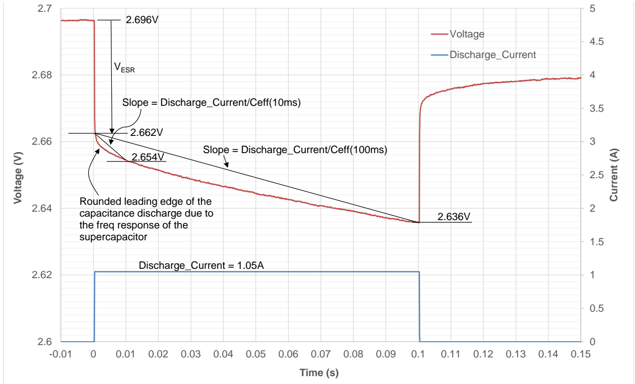
Fig 7: Discharge pulse illustrating the concept of Ceff
