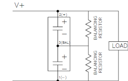
SUGGESTED CONNECTION DETAILS FOR 2 - CELL SUPERCAP
