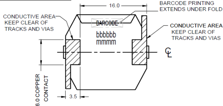
BOTTOM VIEW - G OPTION
