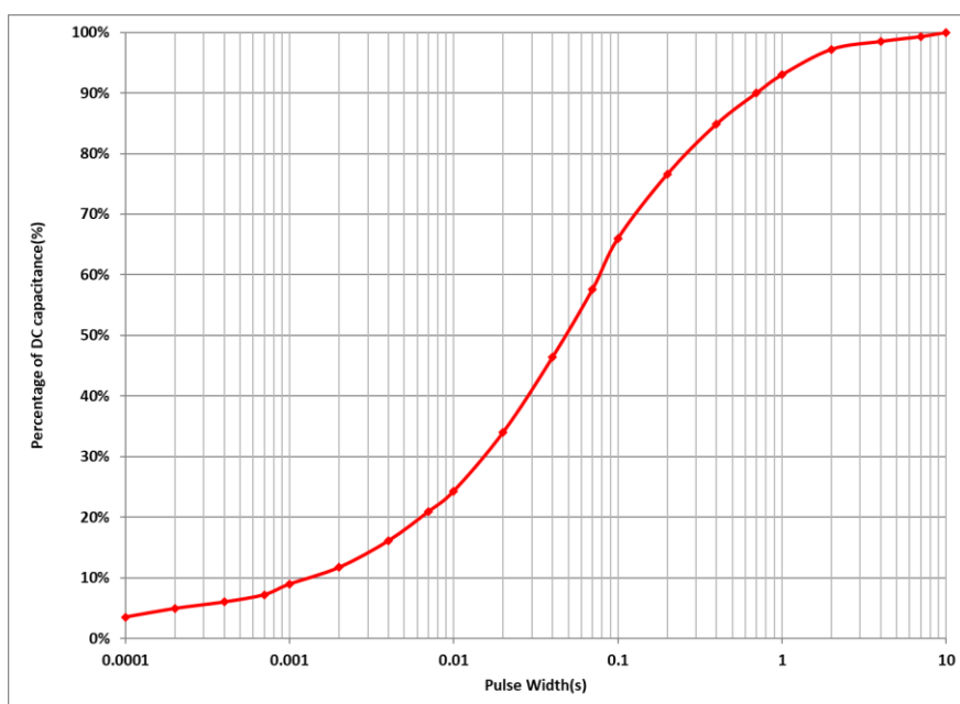
Fig 4: Effective Capacitance
