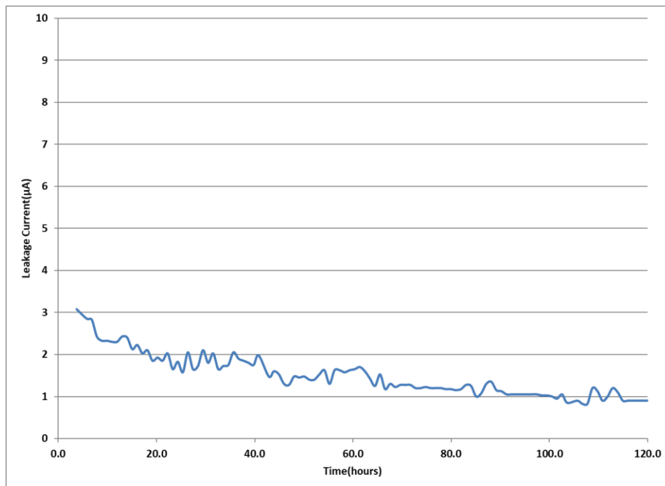
Fig 10: Leakage Current
