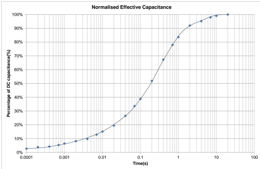
Fig 8: Typical effective capacitance for GY 2.7V series supercapacitors
