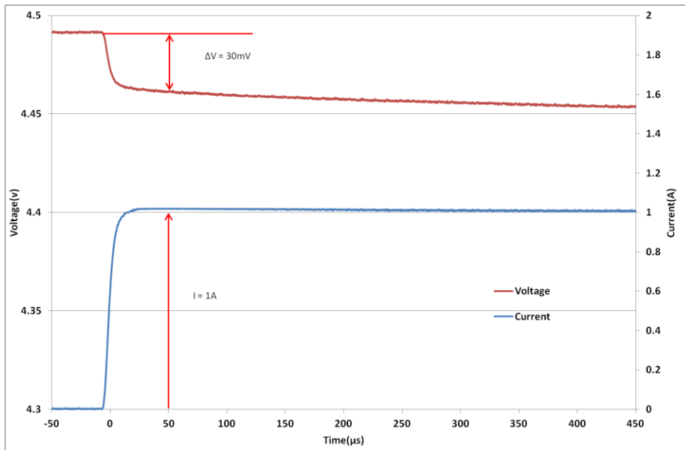
Fig 3: Measurement of ESR for a GW203
