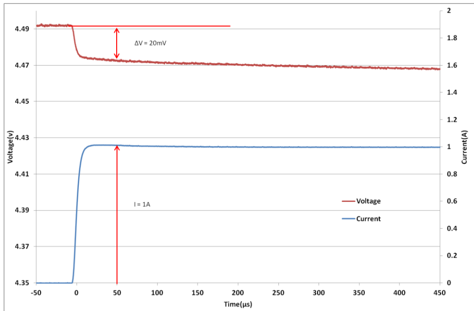
Fig 3: Measurement of ESR for a GS208
