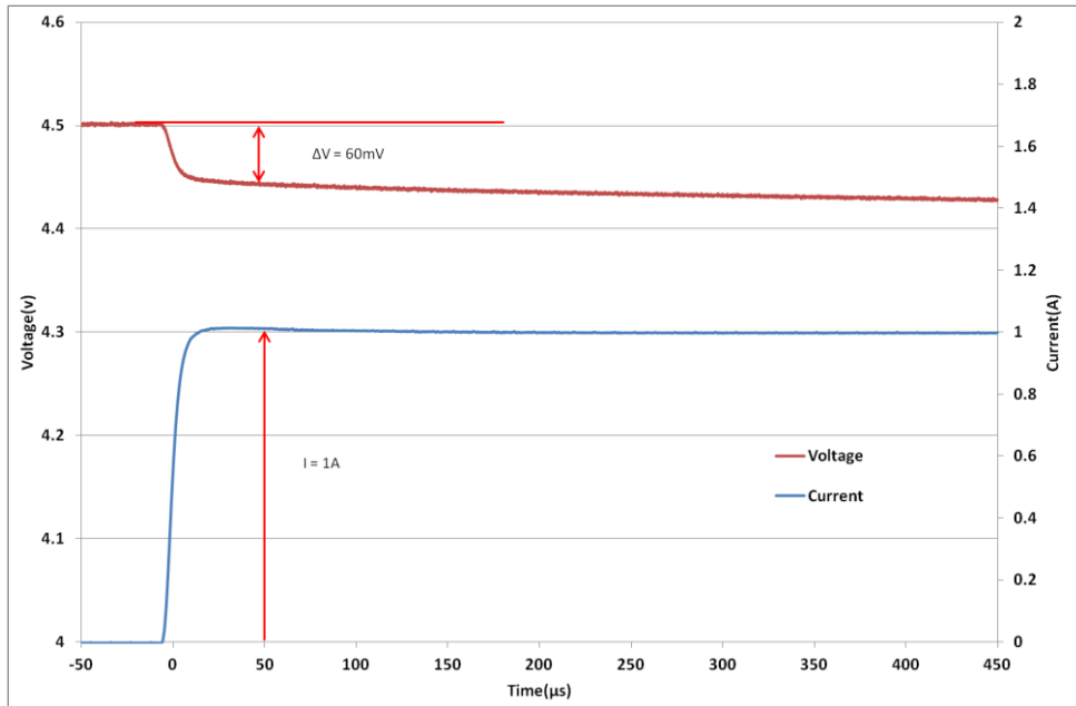
Fig 3: Measurement of ESR for a GA230
