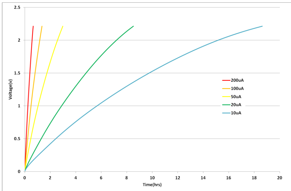
Fig 11: Charging an GA109 with low current
