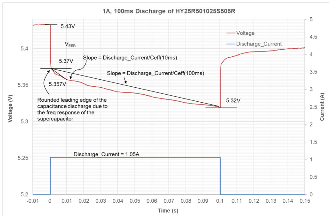
Fig 9: Discharge pulse illustrating the concept of Ceff
