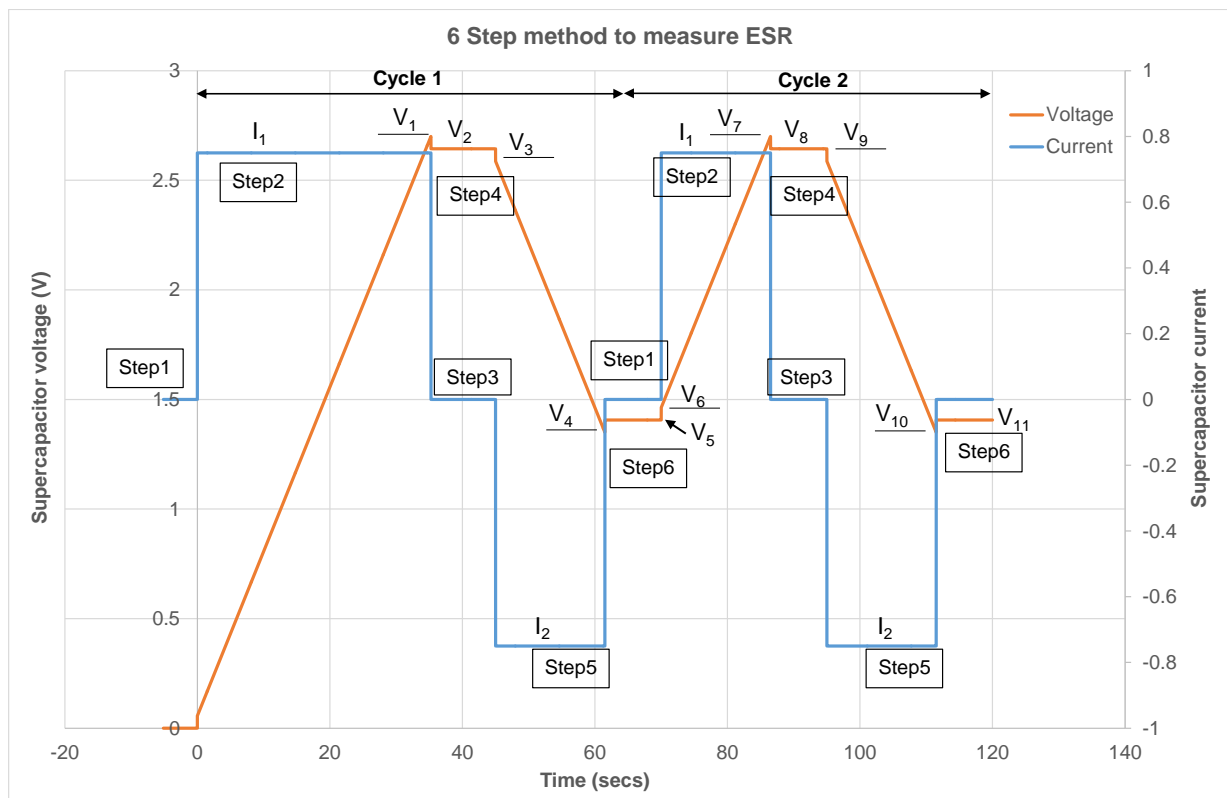
Fig 2: ESR Measurement
