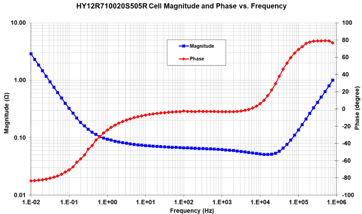
Fig 7: Magnitude and Phase Frequency Response for 5F cell, HY12R710020S505R
