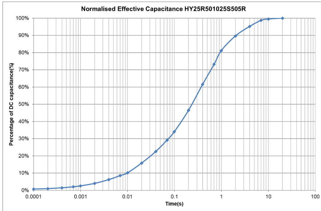
Fig 10: Normalised effective capacitance for HY series supercapacitors
