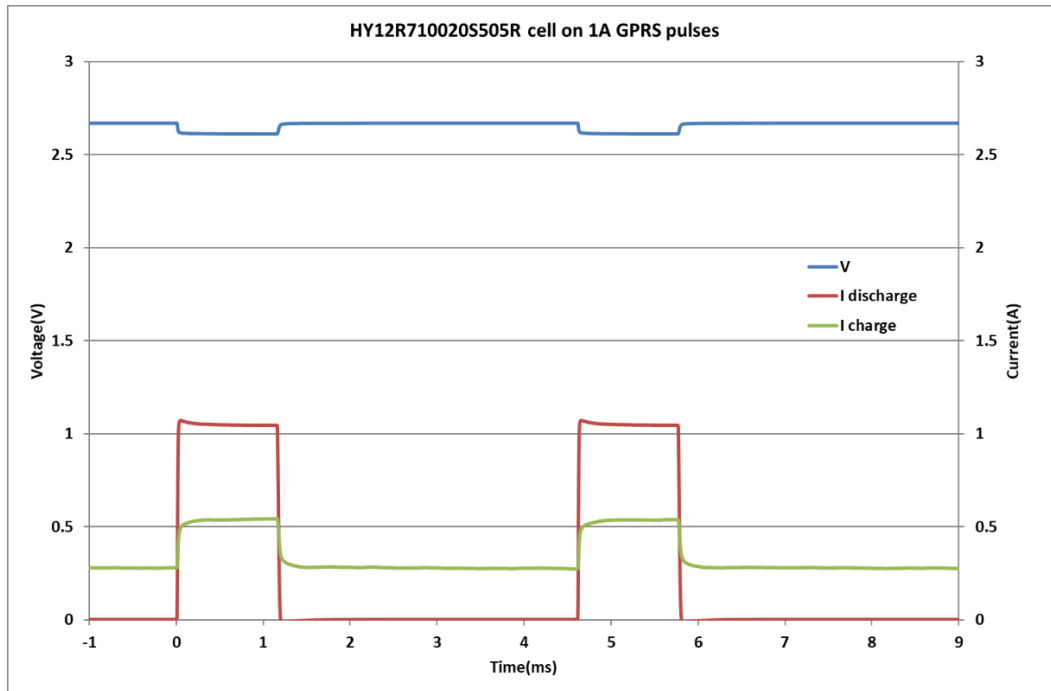
Fig 8: Pulse response of an HY12R710020S505R
