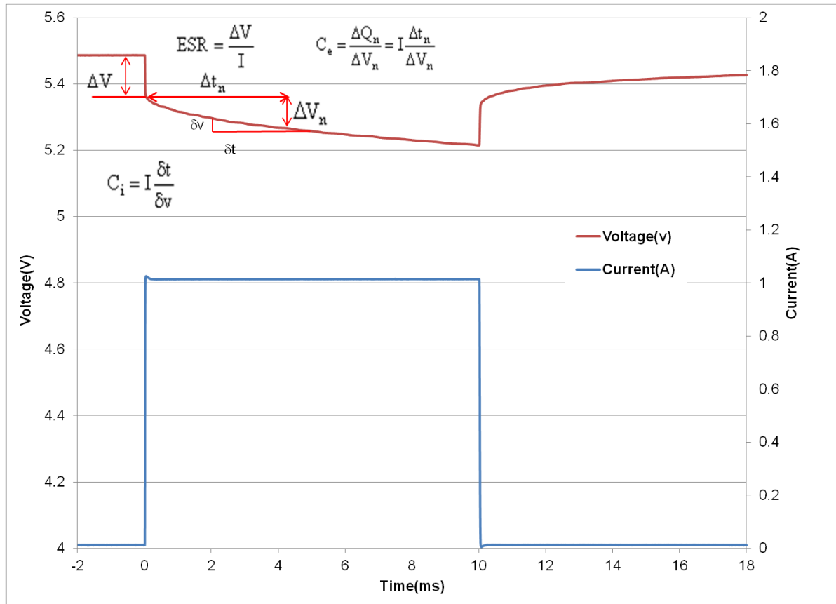
Figure 1: Effective capacitance, instantaneous capacitance and ESR for an HA230
