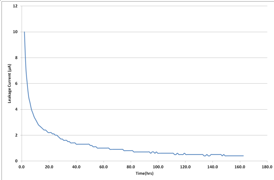
Fig 10: Leakage Current
