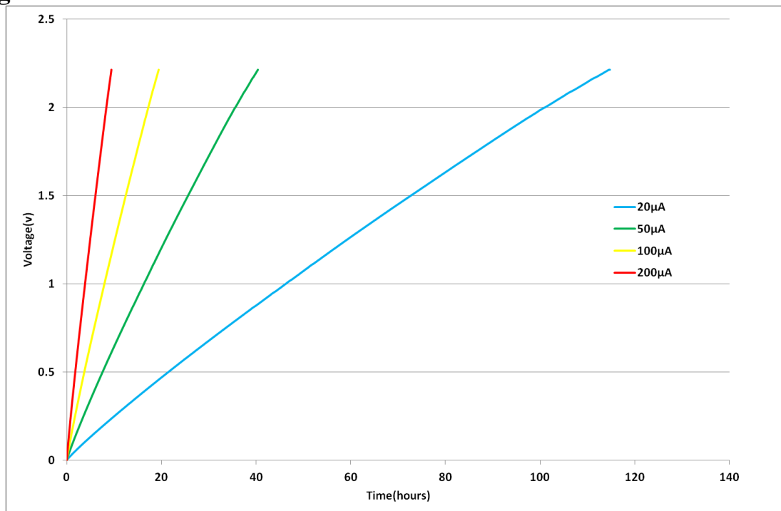
Fig 11: Charging a GS130 with low current
