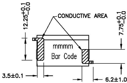
UNDERSIDE VIEW
