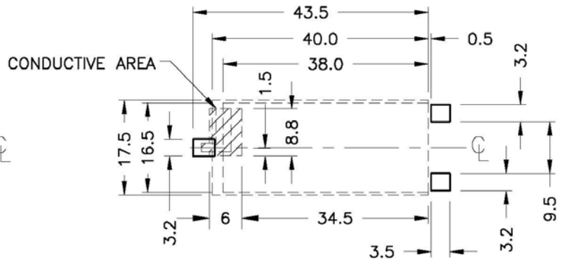
SUGGESTED PAD LAYOUT
